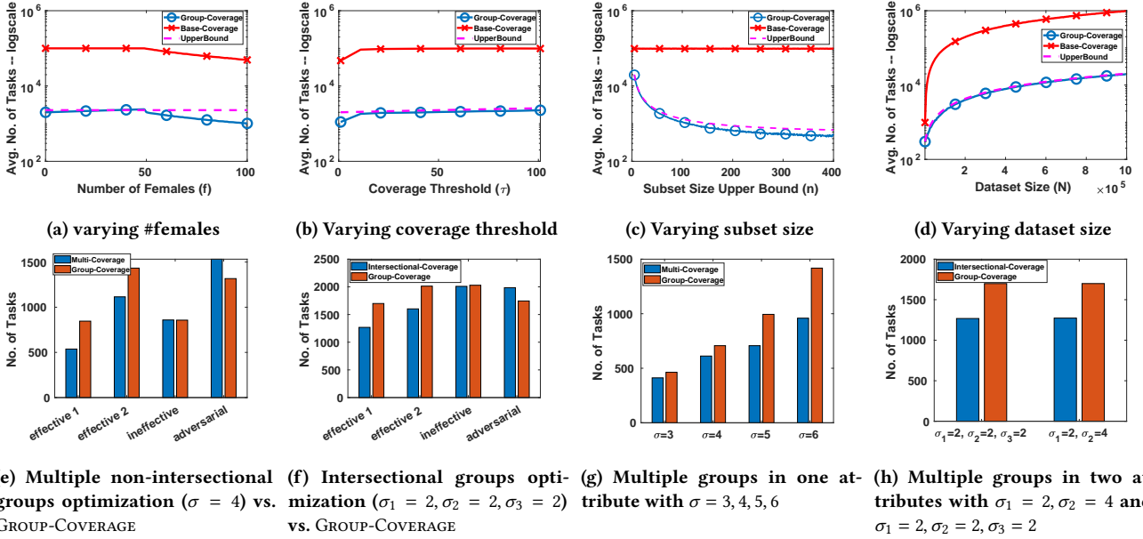
Figure 7: Performance evaluation for GROUP-COVERAGE, MULTIPLE-COVERAGE, and INTERSECTIONAL-COVERAGE algorithms
