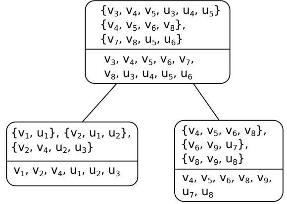
Figure 2: A generalized hypertree decomposition of width 3 for the hypergraph from Figure 1. The boxes are the guarded blocks. In the upper parts the guards are given while the lower parts show the blocks.
