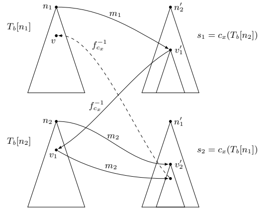
Figure 3: Illustration of the trees and associated nodes used in the proof of Lemma 4.21.
