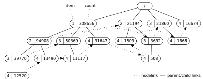
Figure 1: An FP-tree
