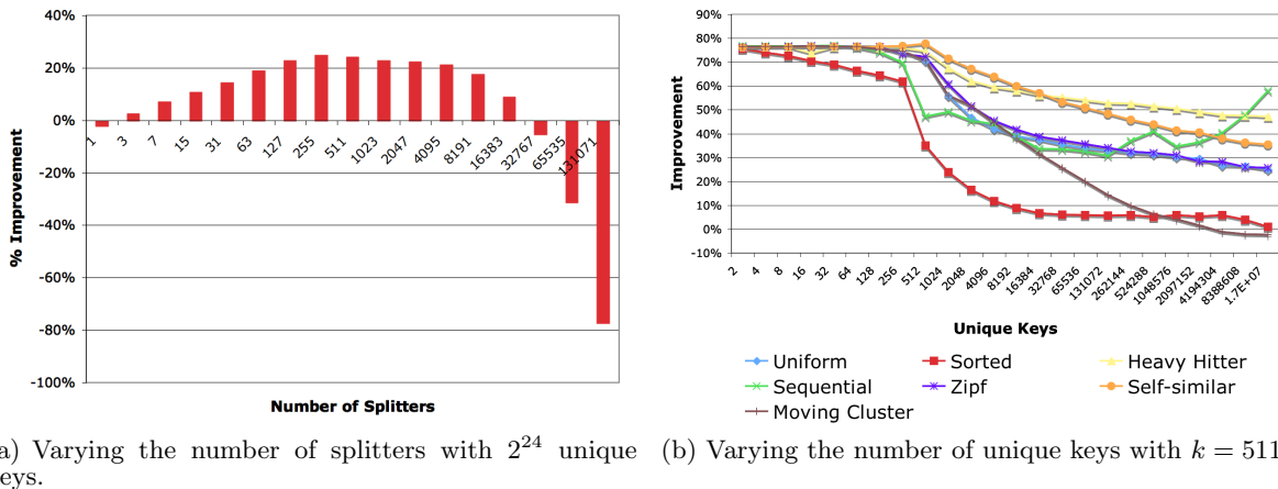
Figure 10: Partition-then-sort improvement over std::sort .
