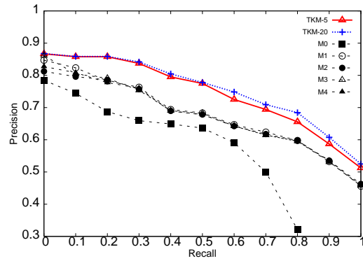
Figure 6: Recall-Precision graphs: TKM and individual measures M0-M4
