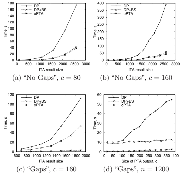
Figure 12: Performance of Exact Algorithms.
