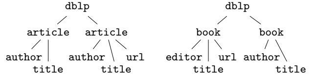
Figure 13: Input sample
