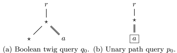
Figure 4: Twig queries.
