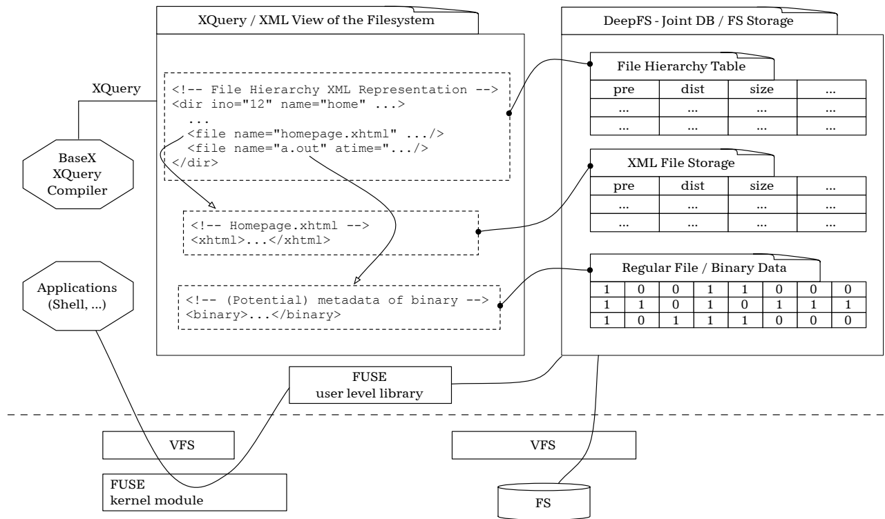
Figure 1: The user level filesystem serves as a joint storage for filesystem and database. Queries against an XML representation of the filesystem are possible as well as conventional filesystem access via the OS.
