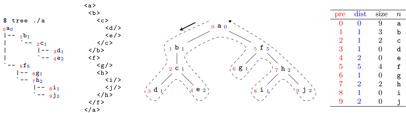
Figure 2: Storing trees (such as file hierarchies, XML documents) in the pre/distance/size encoding.
