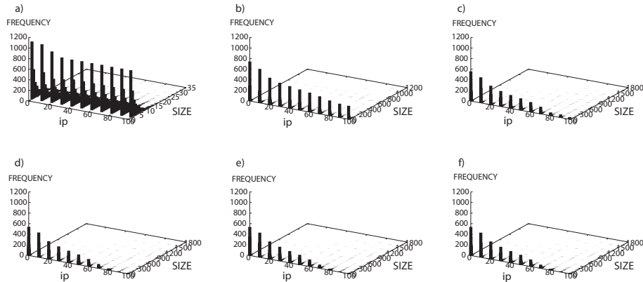
Figure 8: The distribution of synteny block size with respect to ip . l_{max} = 1000 . (a) op = 0 , (b) op = 20 , (c) op = 40 , (d) op = 60 , (e) op = 80 , (f) op = 99 . Synteny blocks of size one are not plotted for clarity.
