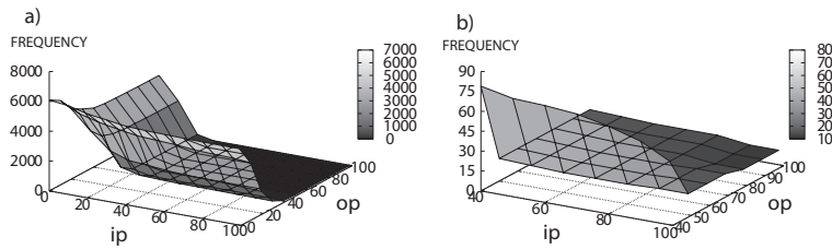
Figure 7: Number of synteny blocks with respect to ip and op .
